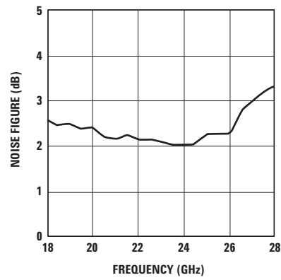
Figure 5. Noise Figure.
