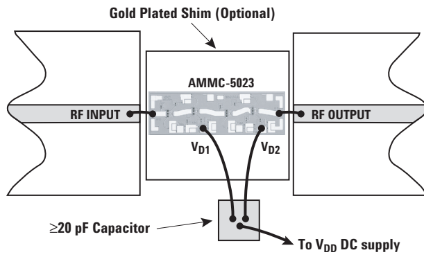
(a) Single DC Drain Supply Voltage.
