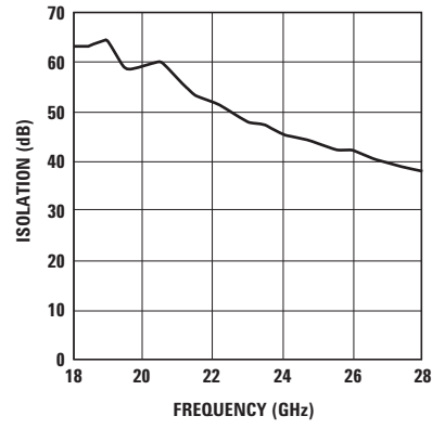
Figure 2. Isolation.
